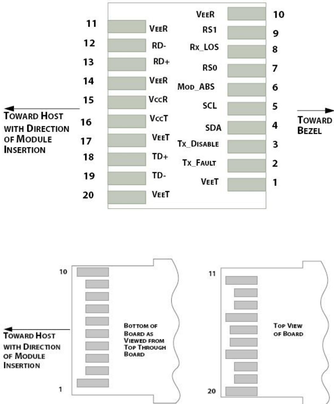
Figure2.Electrical Pin-out Details
