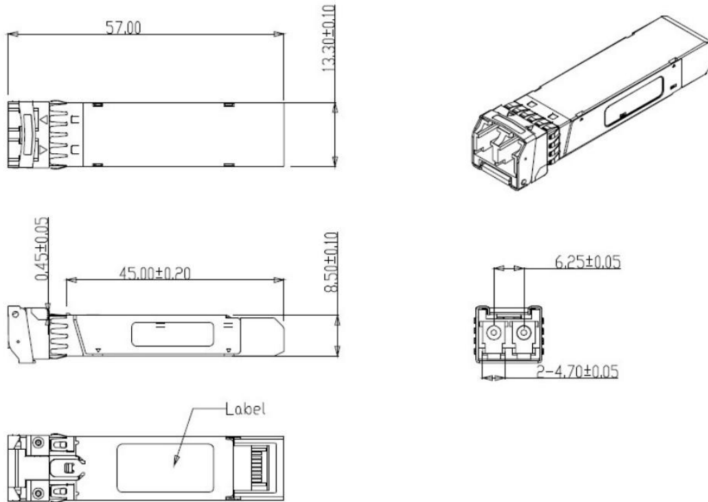
Figure5. Mechanical Specifications
